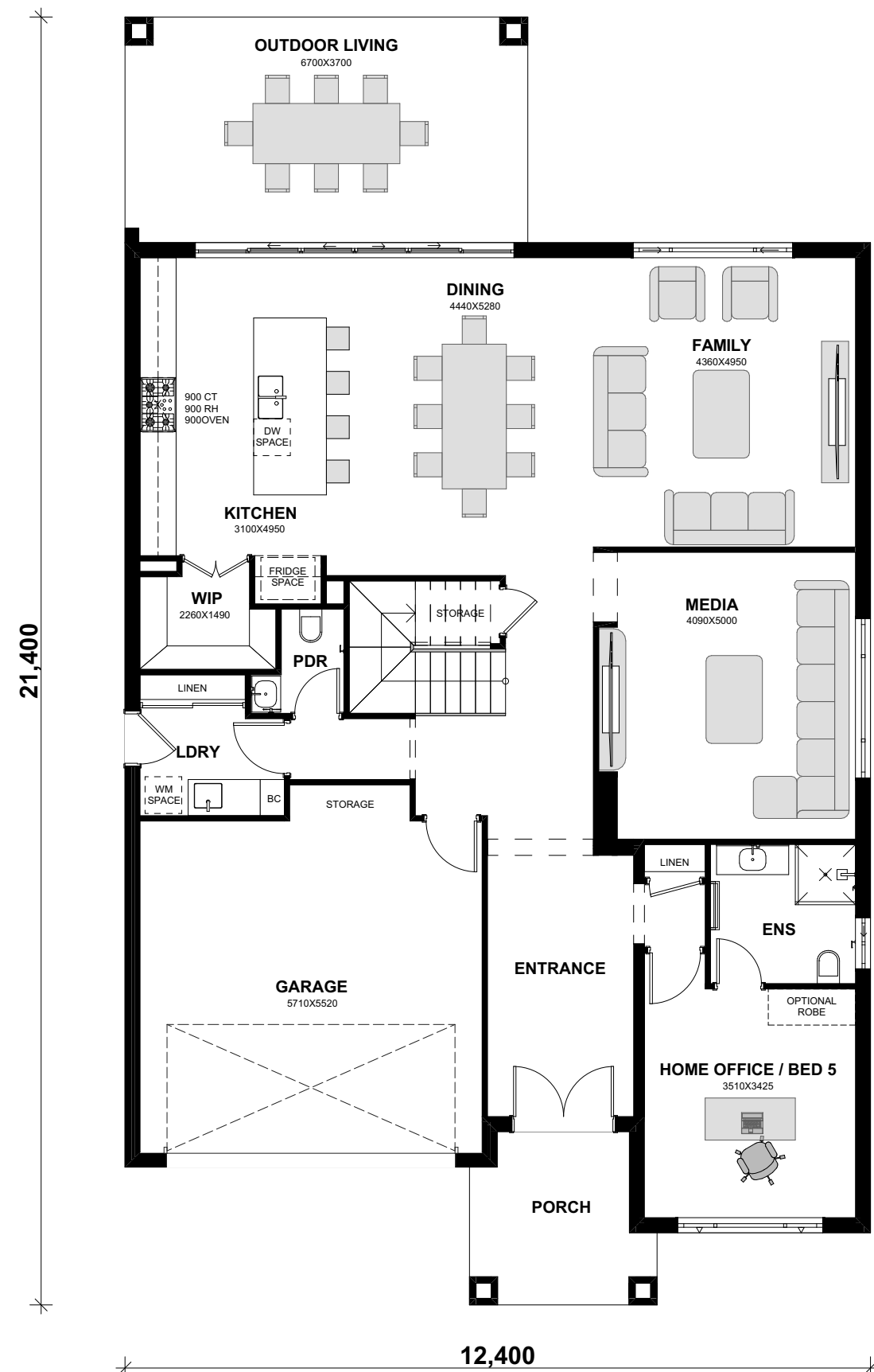
GROUND FLOOR
